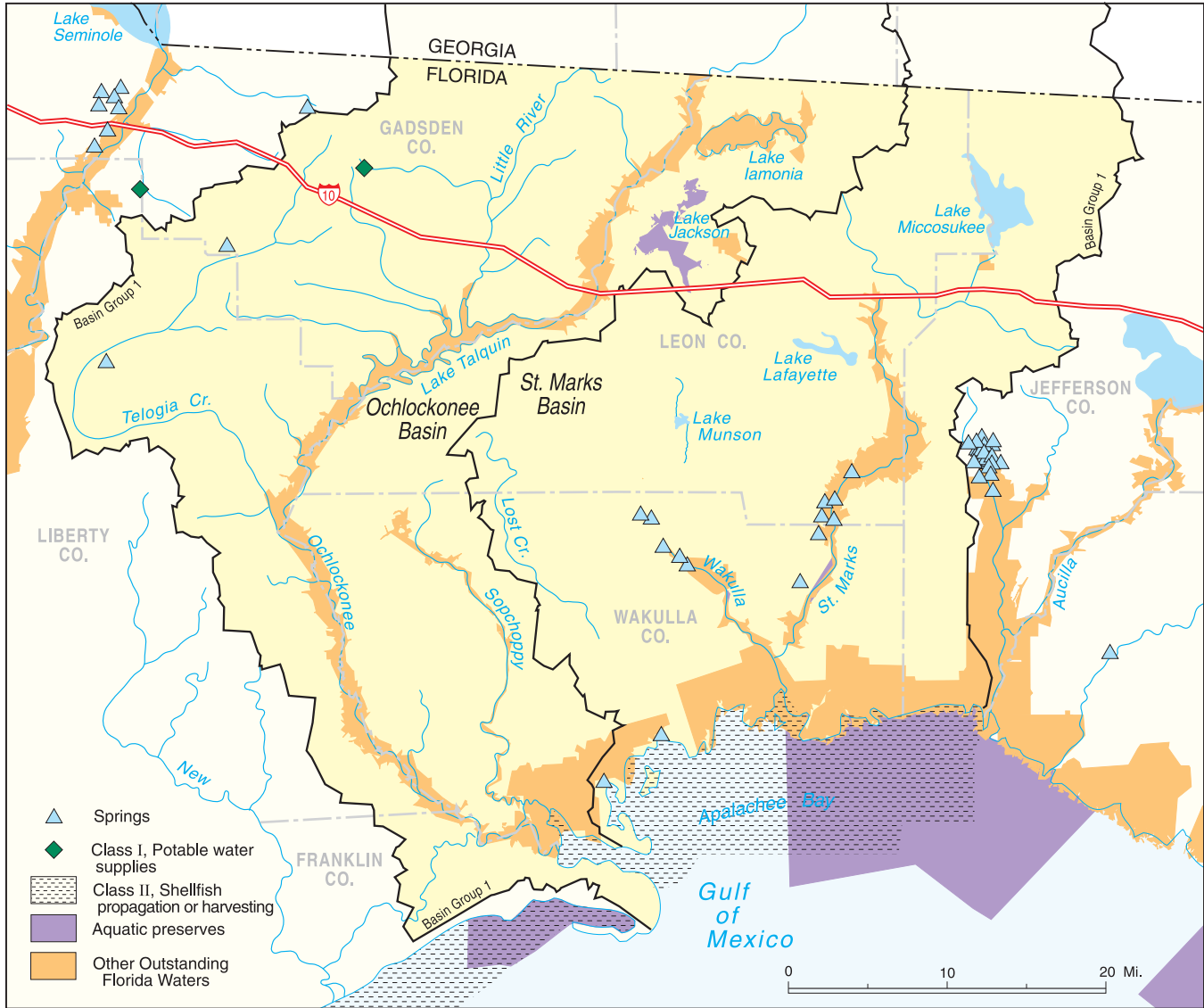
Figure 2.2: Surface Water Resources of the Ochlockonee and St. Marks Basins
