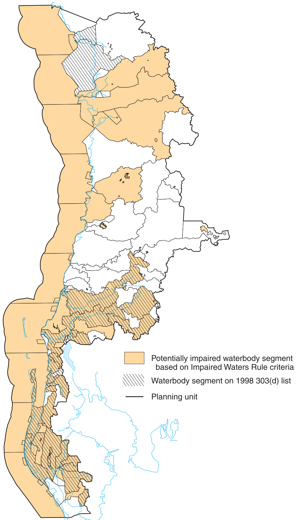
Figure 5.1: Springs Coast Basin Planning List for All Causes of Potential Impairment, with Overlay of 1998 303(d) List
