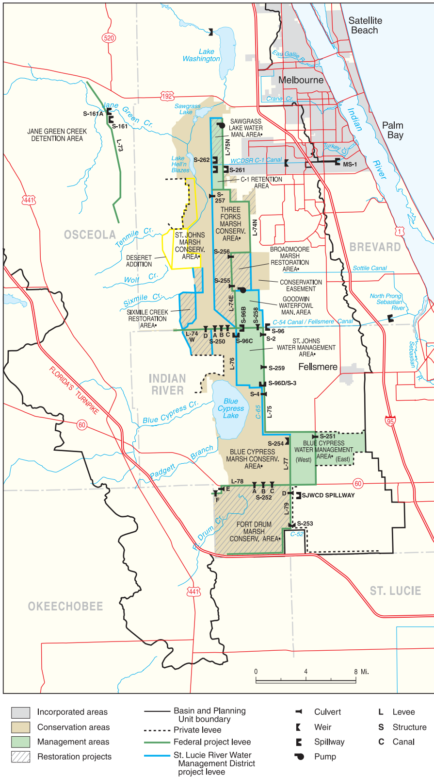
Figure 2.6: Upper St. Johns River Basin Project Area
